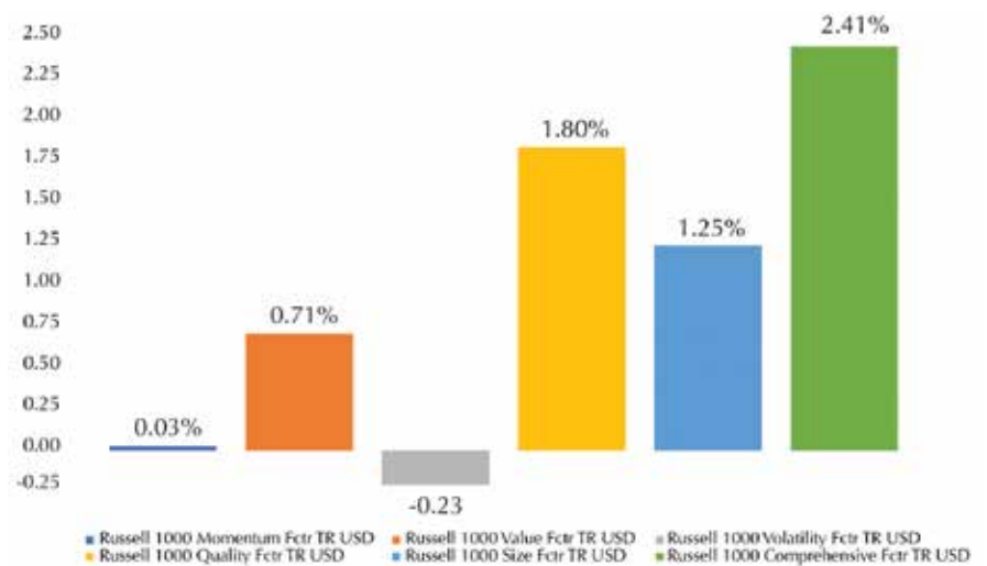
Russell 1000 Factor Excess Returns 2002 to 2023
